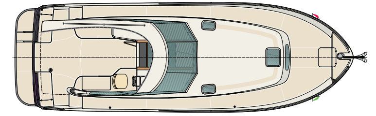
Decklayout
