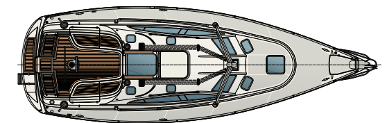
Decklayout
